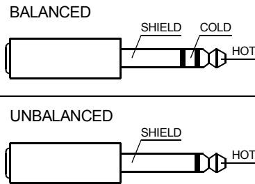
Illustration 2-1: Balanced and unbalanced phone plug
