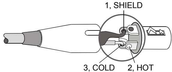
Illustration 2-3: Câbles audio symétrisés (XLR, female)
